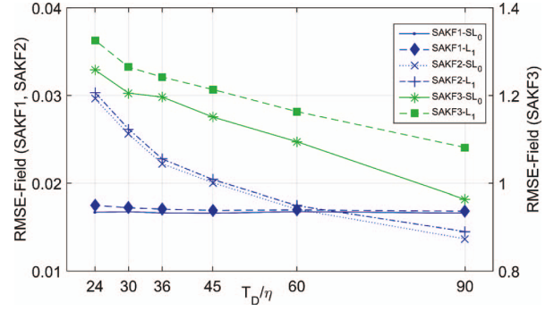
Fig. 9. Steady-state field RMSE. SA-KF algorithm comparison using 16 iterations. Performance averaged over 100 Monte Carlo simulations.
