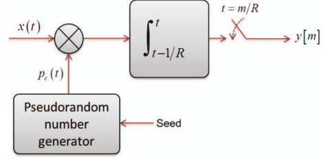
Fig. 2. RD scheme. Adapted from Tropp et al. [17].
