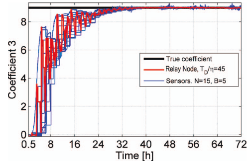
Fig. 14. Example of nonzero coefficient estimate versus time. Sensors and RN gradually reach consensus after about 48 h.
