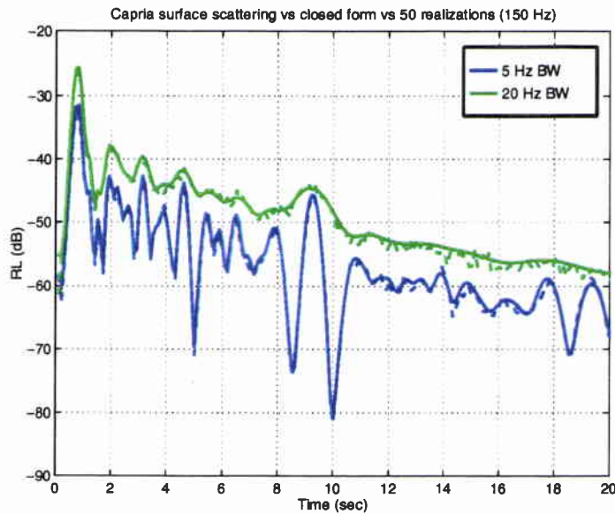
Figure 25 Comparison between the closed form (solid) and Monte-Carlo (dashed) RL at 150 Hz. The excellent agreement for 5 and 20 Hz of bandwidth gives confidence that the closed form expressions are correct.
