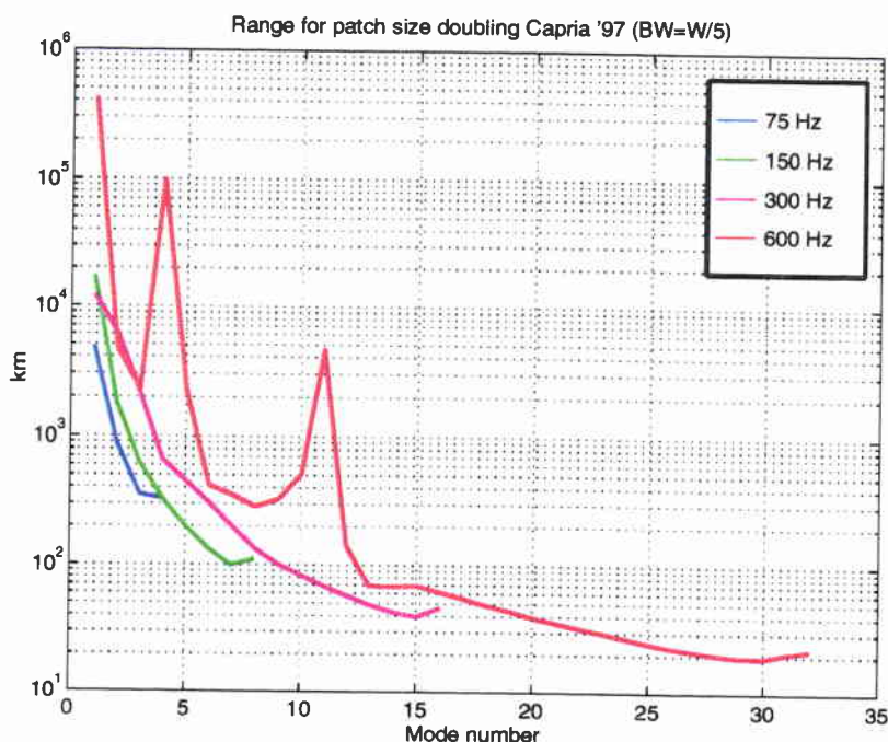
Figure 4 The range at which the bottom patch illuminated by individual modes doubles in size as a function of frequency. For this result, 20% proportional bandwidth of the pulse is assumed. The results indicate that for lower order modes the patch size only doubles after 1000 km, while for higher order modes the patch size can double after as few as 20-40 km.
