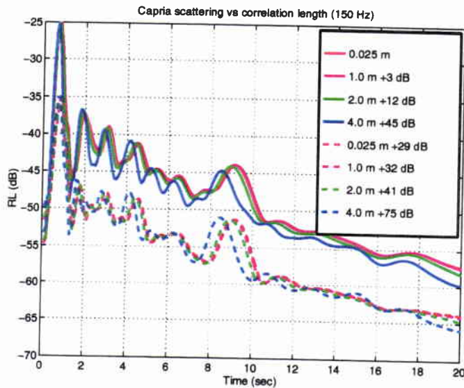
Figure 21 RL as a function of correlation length scale at 150 Hz. Here both the 4.0 and the 2.0 meter correlation length scales have observably different structures from the shorter length scales. Of these, the 4.0 meter correlation length scale effect might be observable in data.
