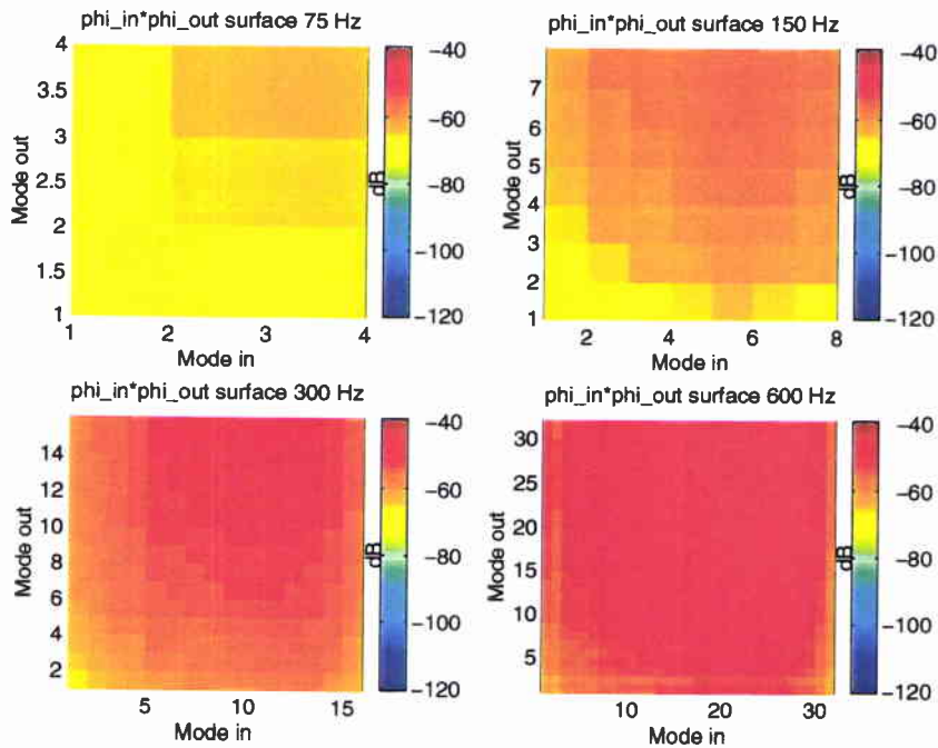
Figure 10 Scattering kernel for rough surface scattering from the water-sediment interface. Lower order modes excite less scattering, and re-radiate less effectively. This kernel is obtained under a perturbation approximation, which for homogeneous boundary scattering would lead to the overall power of the kernels increasing 6 dB per octave. Here the increase is seen to be greater, mostly due to the increasing impedance contrast of the water-sediment interface at higher frequencies.
