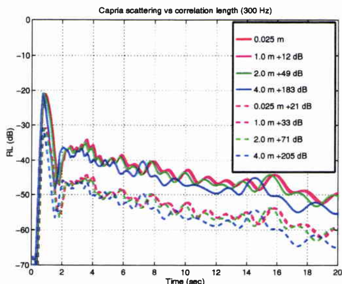
Figure 22 RL as a function of correlation length scale at 300 Hz. As in the 150 Hz case, only the 4.0 meter correlation length scale causes a significant and measurable change in the expected structure of the reverberation.
