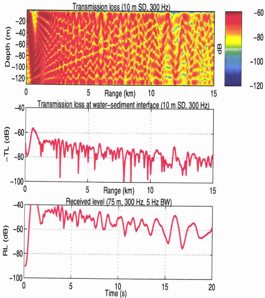
Figure 8 At 300 Hz strong bottom interactions at 6, 10.5, 12 and 13.5 km cause associated spikes in the RL at 8, 14, 16 and 17.5 seconds. Again the scatterers are at the water-sediment interface with a correlation length scale of 0.5 m. The bandwidth is 5 Hz. The coherent interaction between modes for this relatively narrow bandwidth ensures that the underlying CW propagation structure leaves its imprint on the RL. For broader bandwidths, the structure at late time is reduced.
