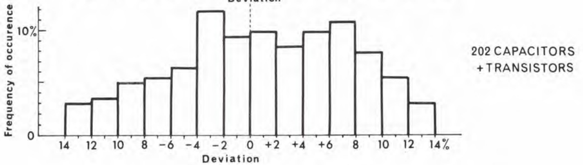
FIG. 6 FREQUENCY DISTRIBUTIONS OF DEVIATIONS FROM QUOTED VALUES
