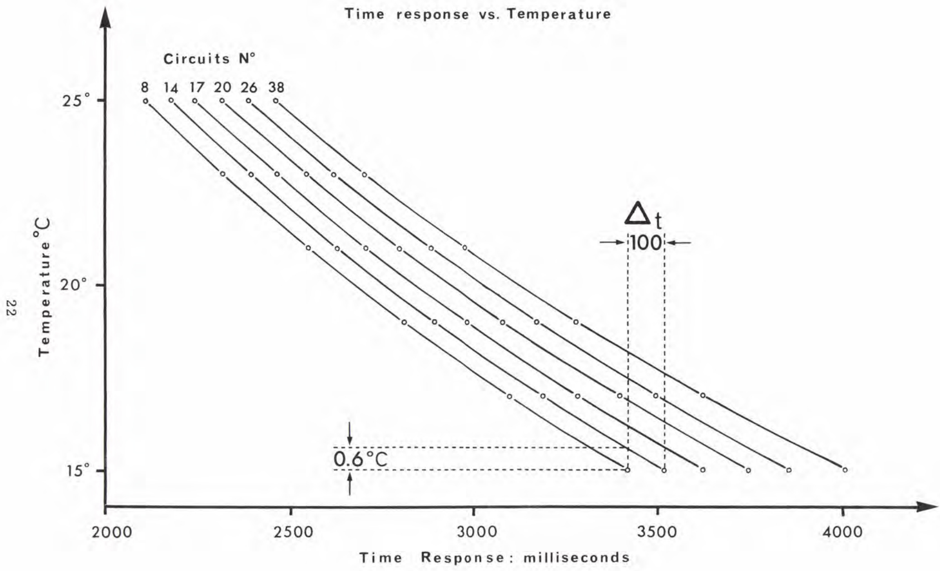
FIG. 5 CALIBRATION CURVES OF THERMOMETERS
