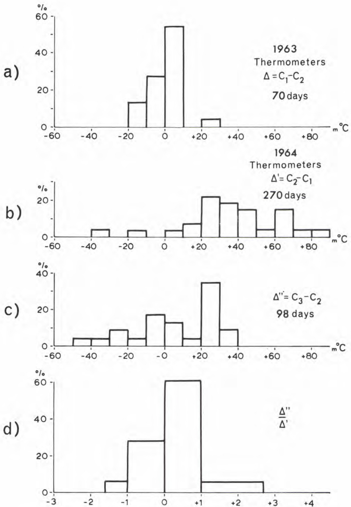
FIG. 7 COMPARISON OF LONG-TERM STABILITY BETWEEN TWO SETS OF THERMOMETERS
