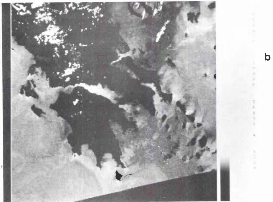
Fig.3a-b The sea-surface temperature images corresponding to Fig. 2.
