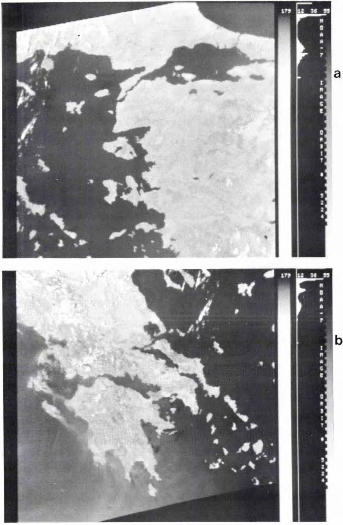
Fig. 2 The images mapped to a Mercator Projection a) centred at 39.5°N, 27°E b) centred at 38°N, 23°E
