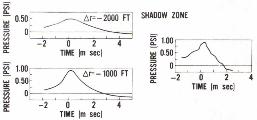
EXAMPLES OF PRESSURE-TIME HISTORIES FOR VARIOUS HORIZONTAL DISTANCES FROM A CONVERGENCE ZONE CAUSTIC
