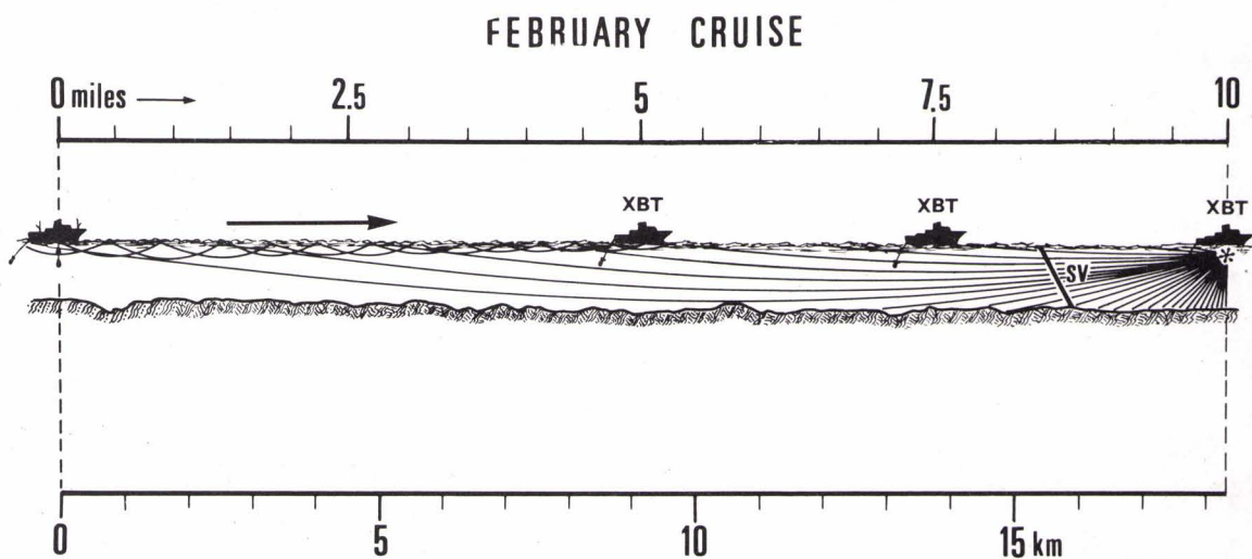
FIG. 5 PLAN FOR THE OCEANOGRAPHIC/ACOUSTIC MEASUREMENTS ALONG THE SHORT RUNS. Each ship to take an XBT every 10 minutes with the firing ship exploding deep and shallow charges every 5 minutes. MARIA PAOLINA stationary at the end of the profile with hydrophones at 5 depths
