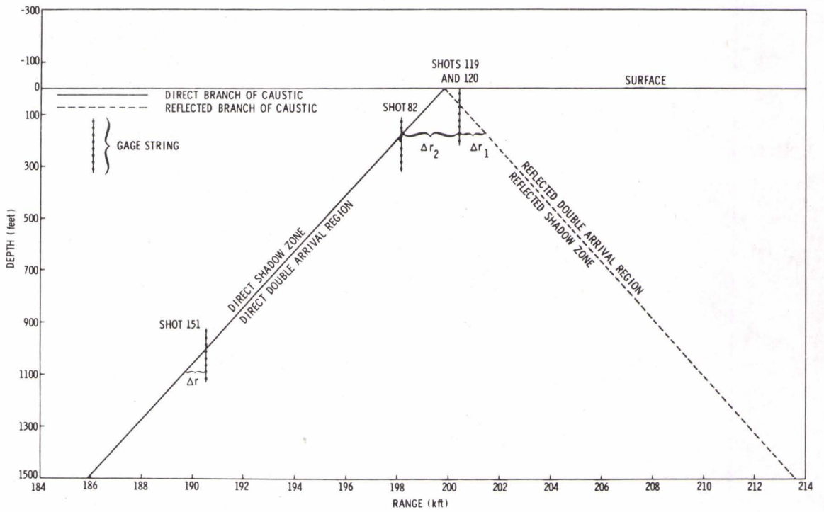
THE POSITION OF THE GAGE STRING WITH RESPECT TO THE CAUSTIC FOR SAMPLE SHOTS
