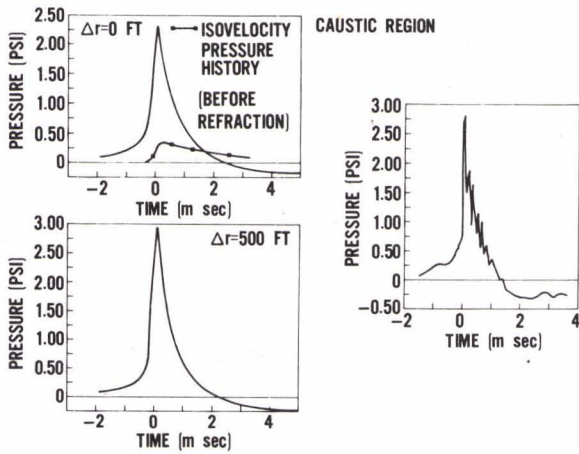
EXAMPLES OF PRESSURE-TIME HISTORIES FOR VARIOUS HORIZONTAL DISTANCES FROM A CONVERGENCE ZONE CAUSTIC
