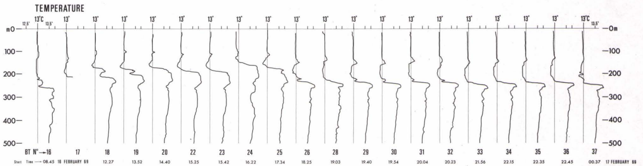
FIG. 2 TEMPERATURE PROFILES TAKEN APPROXIMATELY EVERY HOUR AT ONE STATION IN THE STABILISED COASTAL ZONE (MEDOC 69)
