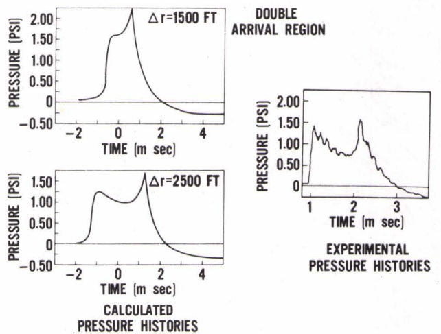
EXAMPLES OF PRESSURE-TIME HISTORIES FOR VARIOUS HORIZONTAL DISTANCES FROM A CONVERGENCE ZONE CAUSTIC
